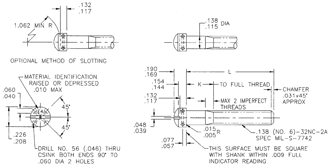
FIGURE 1 - SCREW
